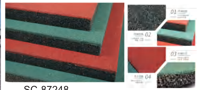
SC-87248 地胶垫 (绿/红/黑) Sports ground rubber mat SIZE:50*50*1.5/2/2.5/3CM 100*100*1.5*2*2.5/3CM QTY:1PC G.W:50CM:14/18/22/26KGS/m² 100CM:14/18/22/27KGS/m² MEAS:50*50*1.5/2/2.5/3CM 100*100*1.5/2/2.5/3CM 建议零售价: ¥325/400/475/550/m²(50*50CM) ¥350/425/500/575/m²(100*100CM)
