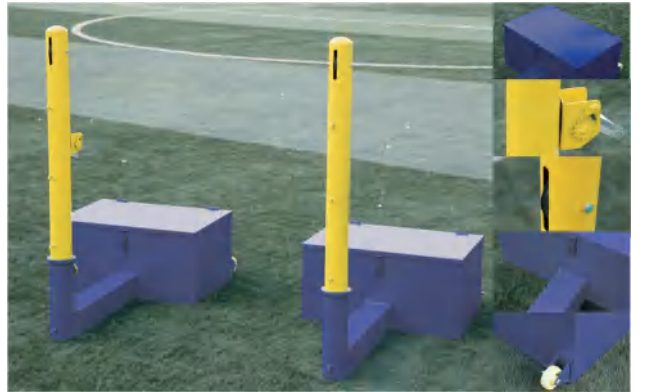
SC-88277 便携移动式网球柱 Portable mobile tennis post 箱体40cmx60cmx30cm QTY:1set=3pkgs (底座2件+立柱1件) G.W: 50kgs/set (配好重量后250kg左右) MEAS:105x60x30cm (底座x2件) 110x18x11 (立柱) 建议零售价: ¥2750/set
