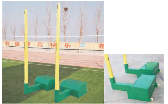
SC-88275 高档大箱排球柱 齿轮升降/把手升降 High-grade big box volleyball post 箱体60x45x30cm QTY: 1set=3pkgs(底座2件+立柱1件) G.W:80kgs/set (配好重量270kgs左右) MEAS:105x60x30cm(底座x2件) 190x23x13cm (立柱) 建议零售价: ¥6000/¥5500/set
